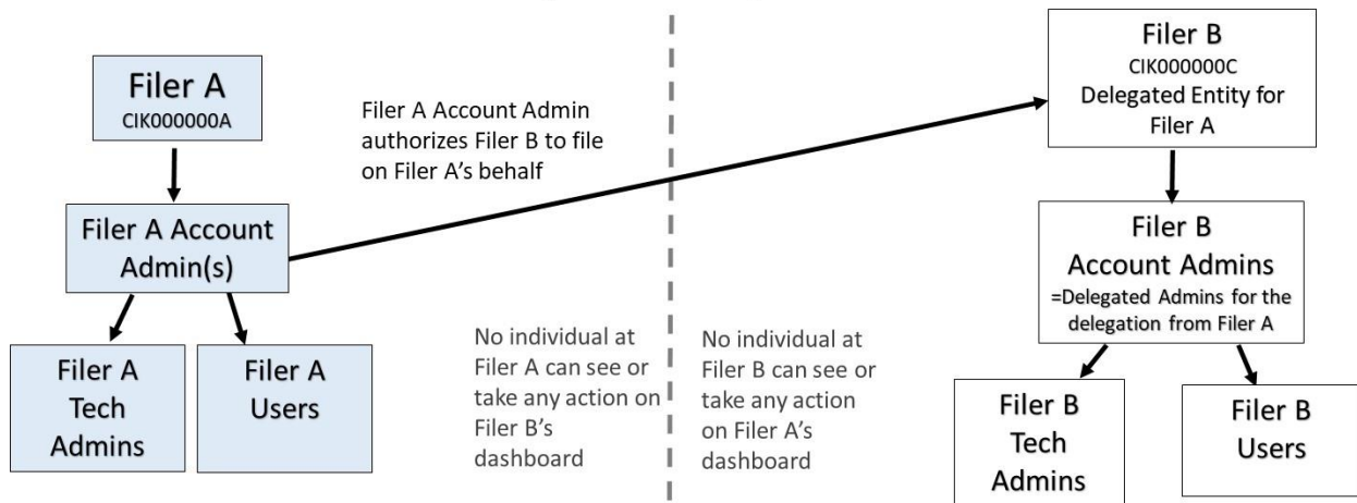
Diagram 3: Delegation
