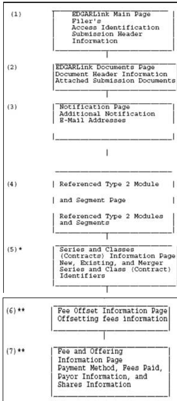
Figure 7-17: Submission Requirements for Electronic Filing
