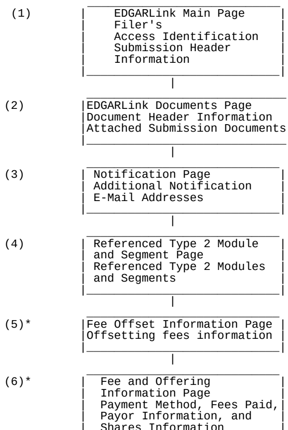
Figure 5-1: Submission Requirements for Electronic Filing
