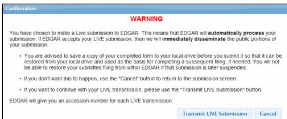
Figure 9-127: Confirmation Screen
