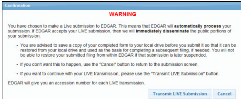
Figure 9-77: Confirmation/Warning Screen
