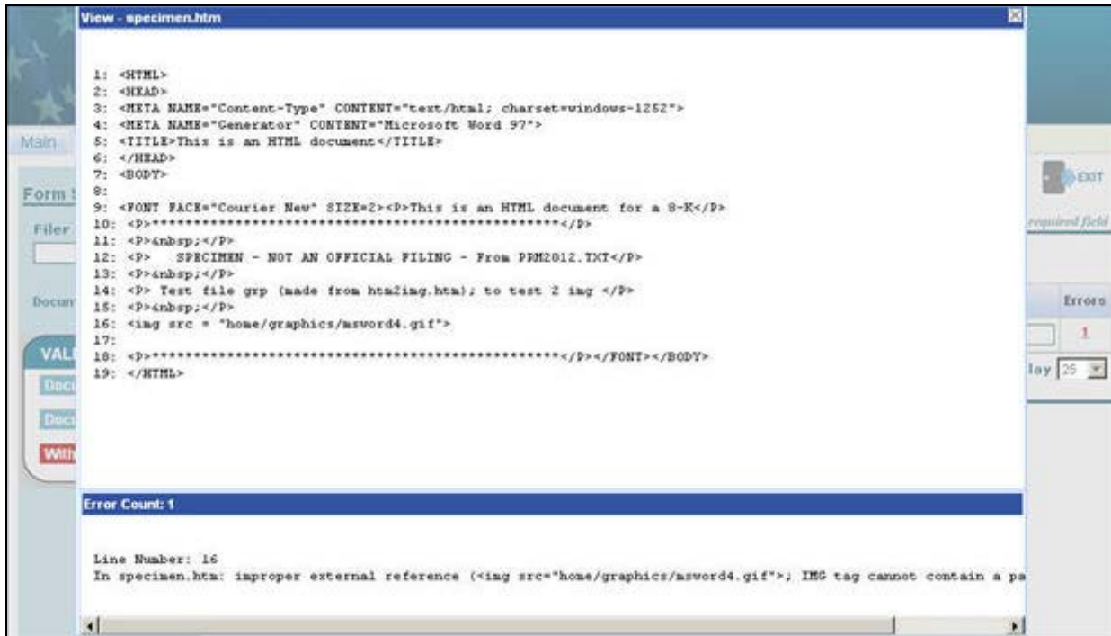
Figure 7-39: Document Validation Window
