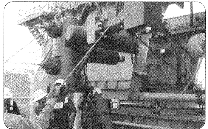
Dry tree installation – South China Sea
