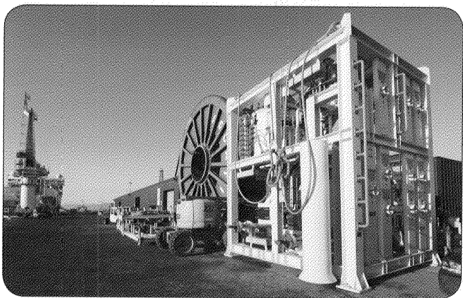
HIPPS manifold for installation in the North Sea
