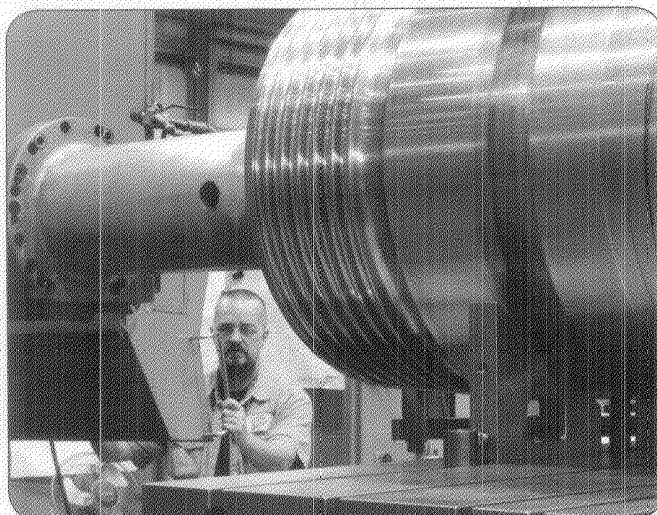
Machining of the SS-20 BigBore II-H wellhead with SDX locking profile
