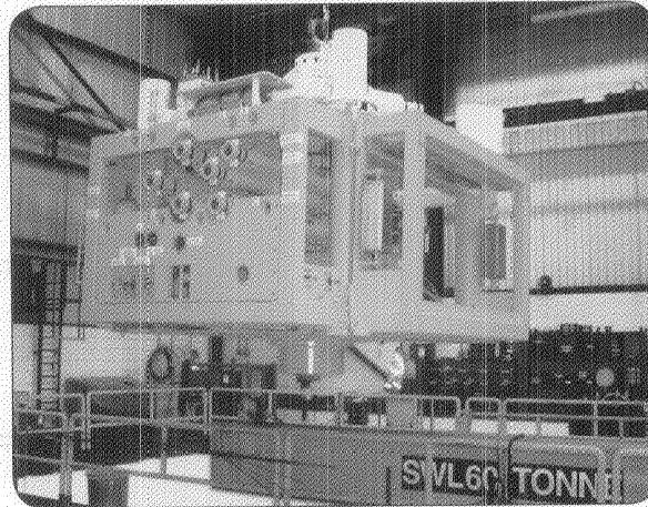
Subsea tree in Assembly, Aberdeen, Scotland
