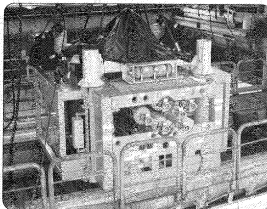
Subsea tree installation
