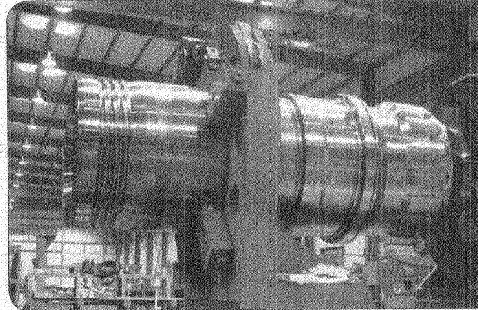
Finish machining of a subsea wellhead, Houston, Texas
