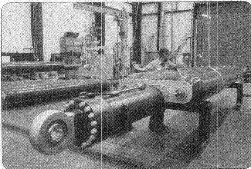
Production riser tensioners in Final Assembly, Houston, Texas
