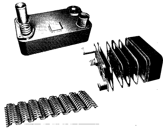
Brake Retarder Cooler Used for on- and off-highway vehicles
