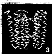
1. HCV p7 pentamer (side view); red: serine, yellow: histidine, green: threonine; 2. HCV p7 pentamer (view from top); 3. Same as number 1 with the United Therapeutics glycochemistry compound docked (side view); 4. Same as number 3 with the United Therapeutics glycochemistry compound docked (view from top)
