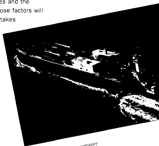
The Energy 13501, the first proprietary double-hulled tank barge built by HOS, on sea trials in March 2005.
