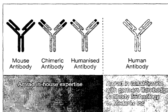
Figure 3: Different types of therapeutic antibodies
