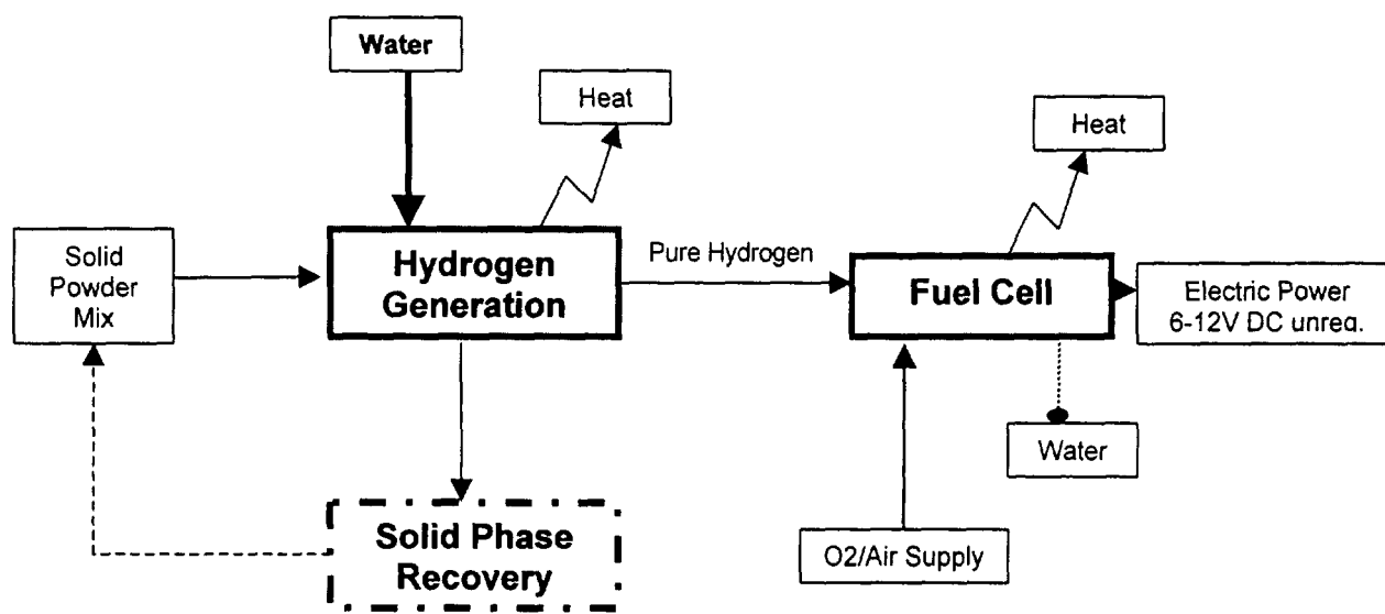
Figure 1: Integrated Fuel Cell with GHTI Hydrogen Generator
