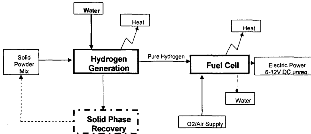
Figure 1: Integrated Fuel Cell with GHTI Hydrogen Generator
