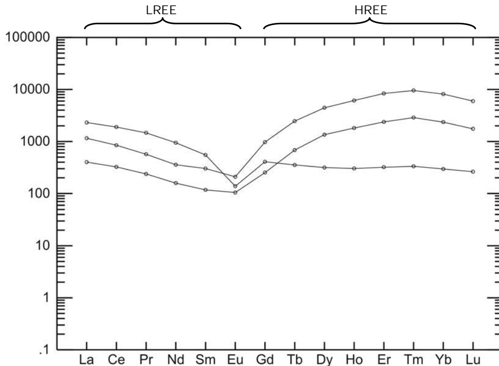
Figure 9.3 – Chondrite-normalized REE diagram for Snake Center (after Taylor and McLennan, 1985). Only mineralized grab samples (>0.17% REE) were plotted.
