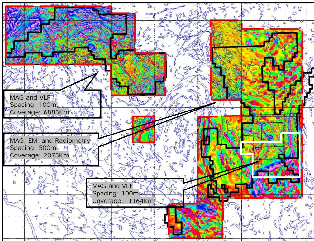
Figure 10.1 – Coverage of the Kipawa property by airborne geophysical surveys conducted by Aurizon in 2006-2007 (Modified from Lafond and Demers, 2008).
