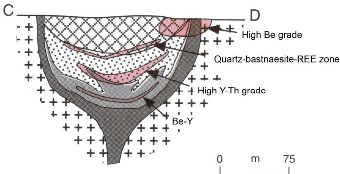
Figure 8.4 – West-east section through mineralization in the northern T Zone at the Thor Lake deposit (Modified from Trueman et al, 1988; and Richardson and Birkett, 1996).
