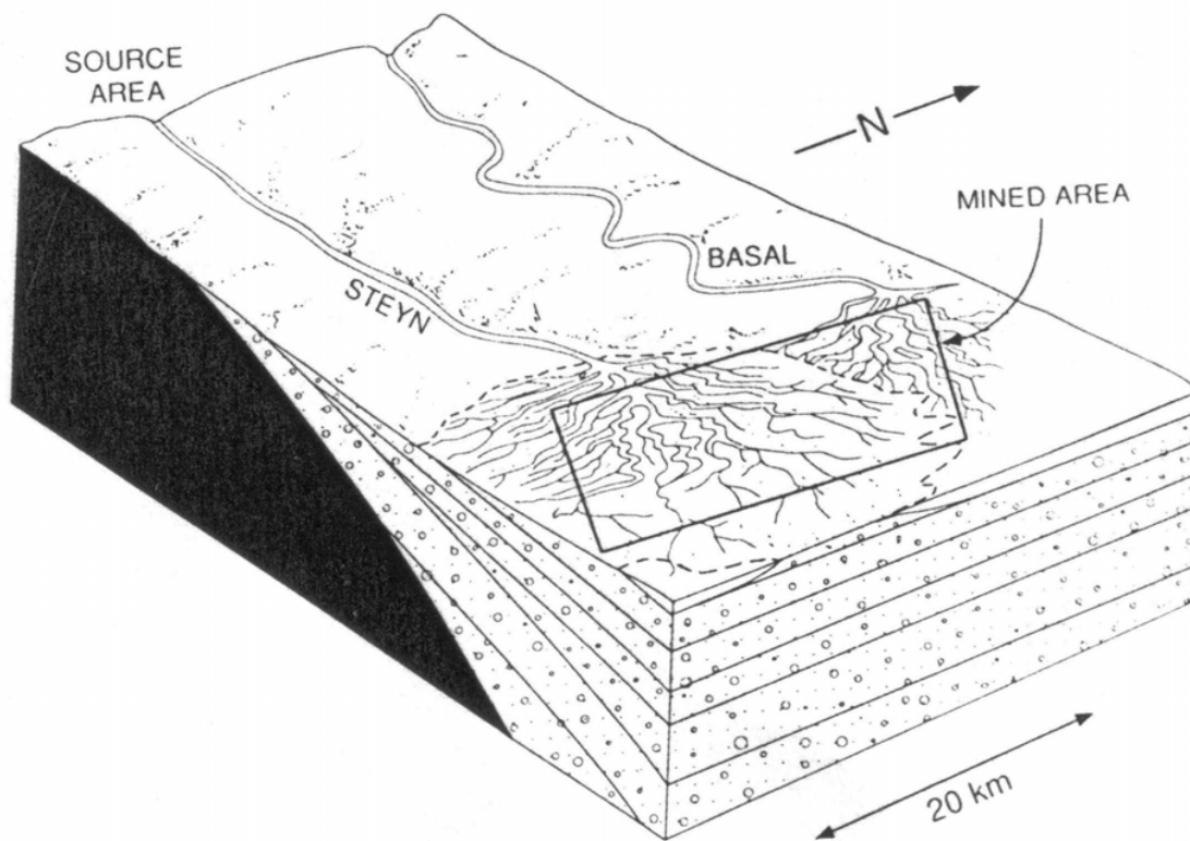
Figure 8.2 – Delta model for deposition of some Witwatersrand paleoplacers (Source: Roscoe and Minter, 1993).
