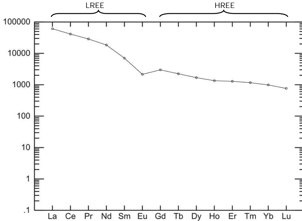
Figure 9.4 – Chondrite-normalized REE diagram for Snake South (after Taylor and McLennan, 1985). The plot represents the single mineralized grab sample from the showing (>0.17% REE).
