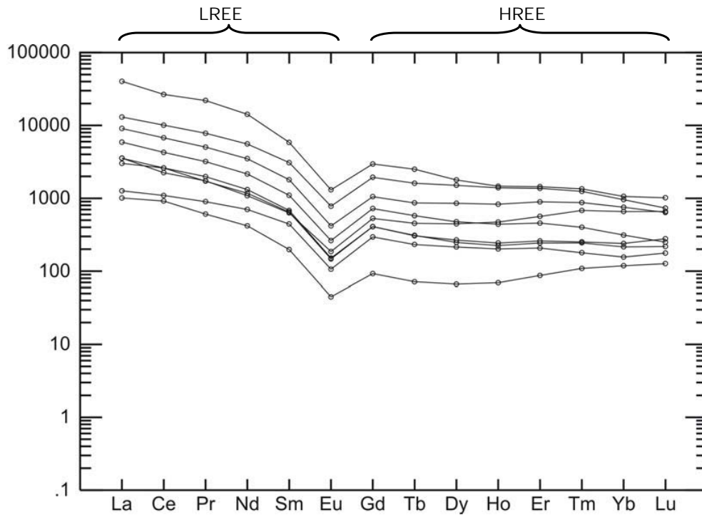
Figure 9.6 – Chondrite-normalized REE diagram for the Eagle showing (after Taylor and McLennan, 1985). Only mineralized samples (>0.17% REE) were plotted.
