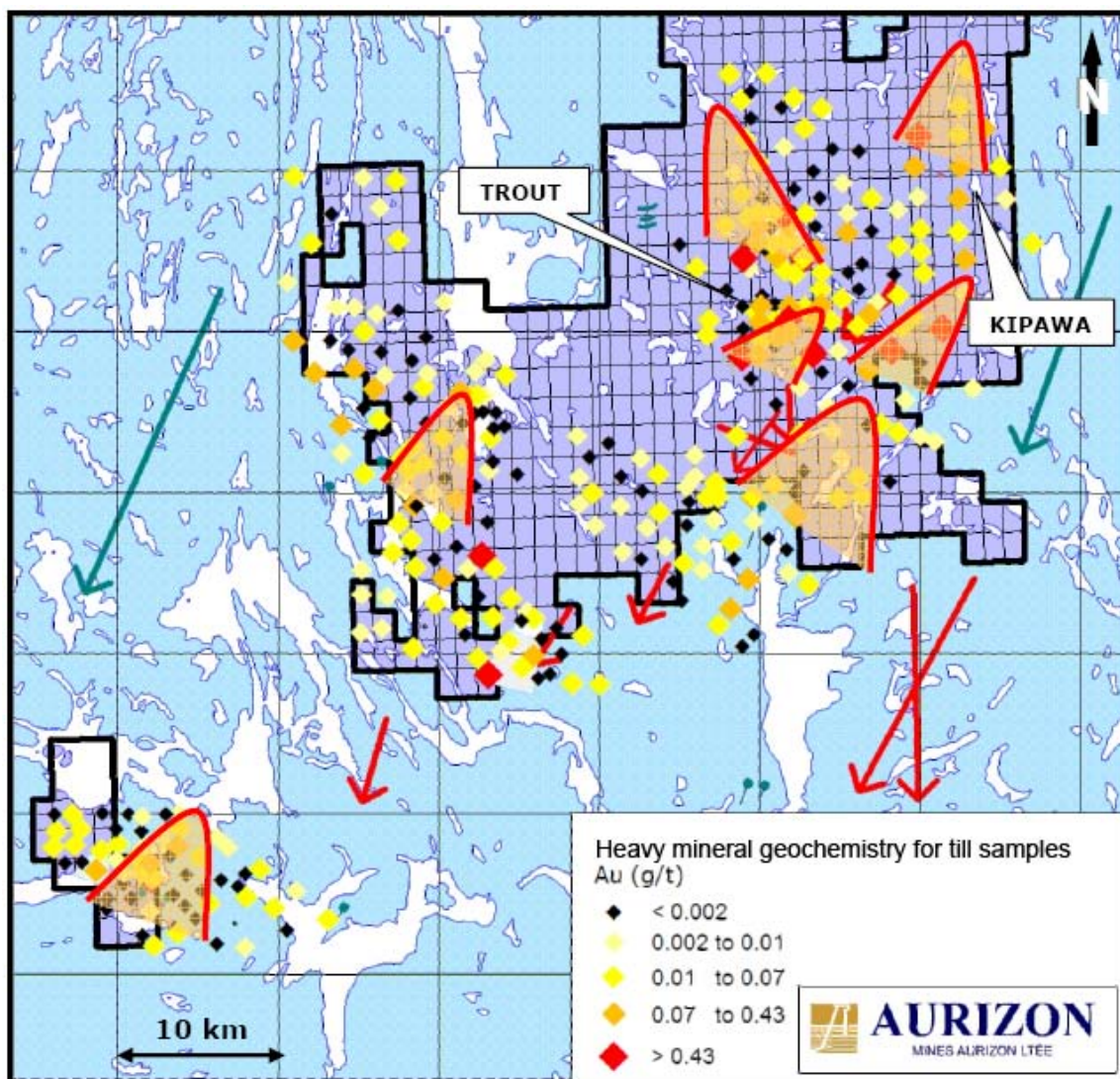
Figure 10.4 – Glacial dispersion trails (in red) and auriferous geochemical results for heavy mineral concentrates from till samples collected on and around Block “S”, the southern part of Block “E”, Kipawa property (Source: Lafond and Demers, 2008).
