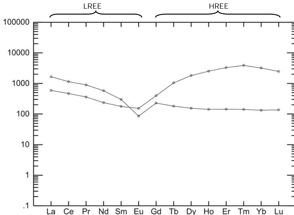
Figure 9.2 – Chondrite-normalized REE diagram for Snake North (after Taylor and McLennan, 1985). Only mineralized grab samples (>0.17% REE) were plotted.
