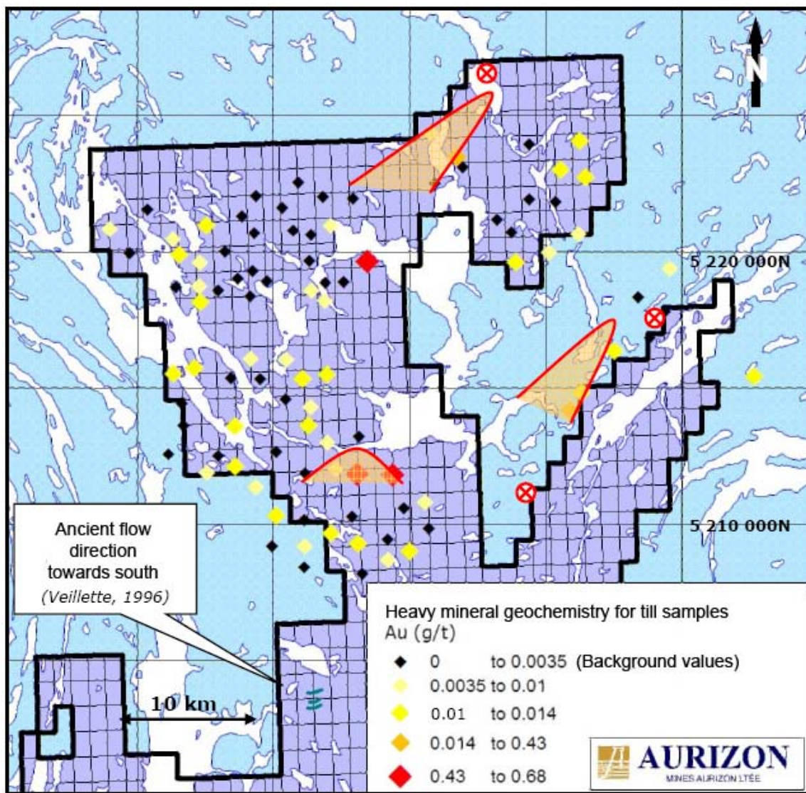
Figure 10.5 – Glacial dispersion trails (in red) and auriferous geochemical results for heavy mineral concentrates from till samples collected from the northern part of Block “E” and its immediate vicinity, Kipawa property (Source: Lafond and Demers, 2008).
