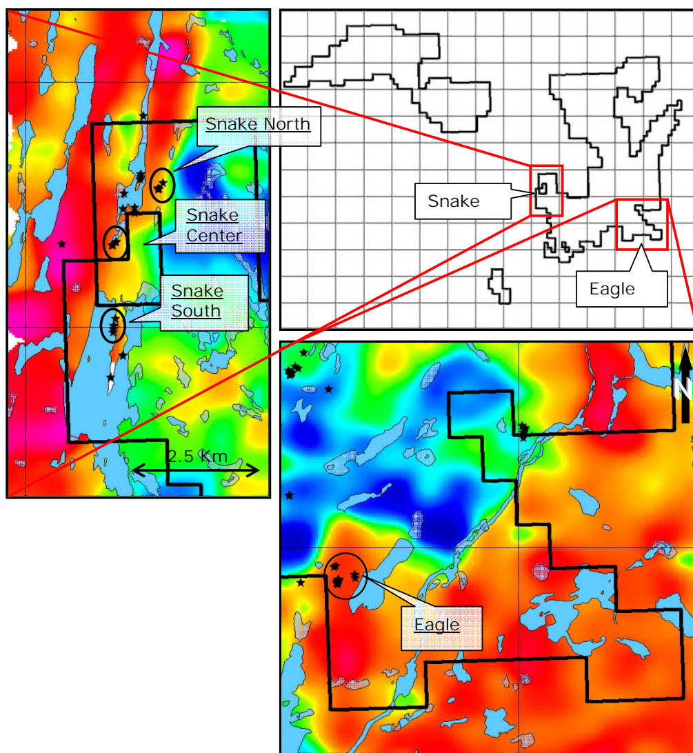
Figure 9.1 – Location of the Snake and Eagle showings within the Kipawa property. Background is radiometric surveys (Modified from Lafond and Demers, 2008).
