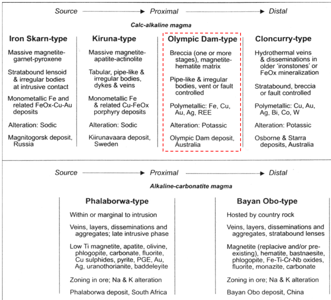
Figure 8.6 – Classification of magmatic-hydrothermal iron oxide deposits and related Cu-Au deposits (Source: Corriveau, 2007 after Gandhi, 2004)
