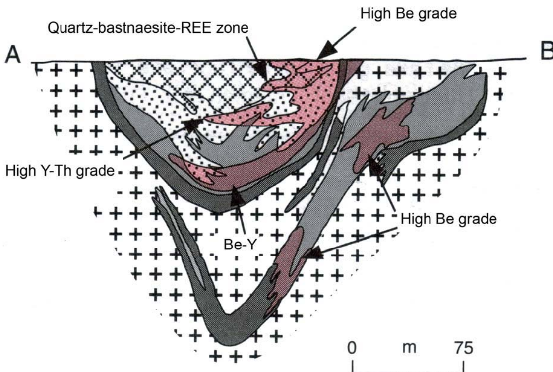
Figure 8.3 – North-south section through mineralization in the northern T Zone at the Thor Lake deposit (Modified from Trueman et al, 1988; and Richardson and Birkett, 1996).
