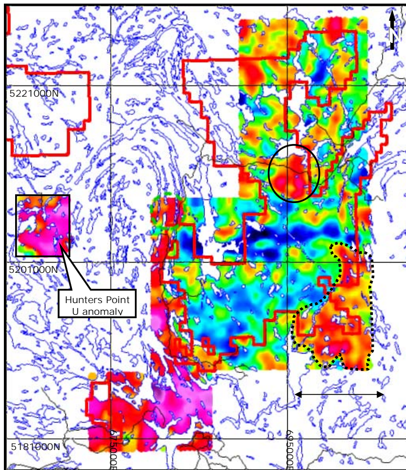
Figure 10.3 – Filtered radiometric data showing the contour (dotted line) of the radiometric high corresponding to the Kipawa Alkaline Complex. Another radiometric high is circled, several kilometres NW of the complex in the central part of Block “E”. Modified from Lafond and Demers, 2008.
