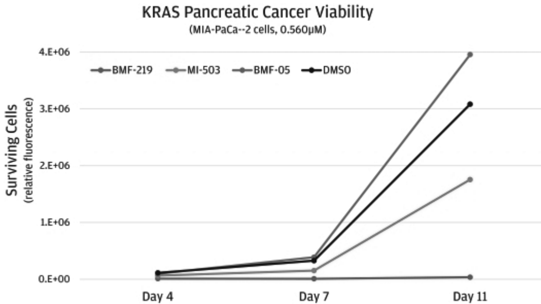
Representative cell survival time course from a KRAS mutant pancreatic cancer model (MIA-PaCa-2 cell line, 0.56 \mu M doses) shows relative effect of the covalent inhibitor BMF-219 versus reversible inhibitors MI-503 and BMF-05
