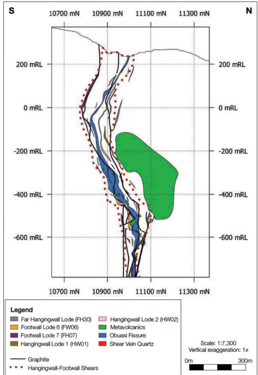
A typical schematic representation of the deposit in local grid, elevation in mRL*
