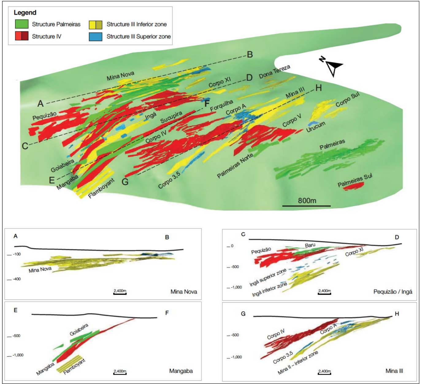
Plan view of the underground orebodies at Serra Grande (top), with sections across the individual orebodies (bottom four sections), elevation in metres below surface*
