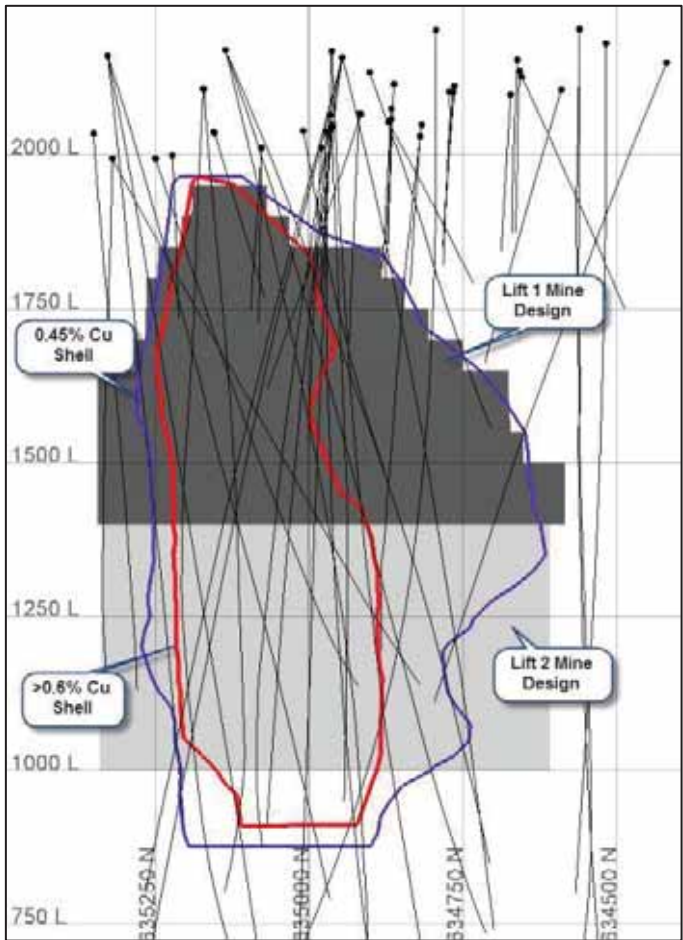
Figure 6. Nuevo Chaquiro Hypothetical Lifts in Grey behind Grade Shells (View to East)
