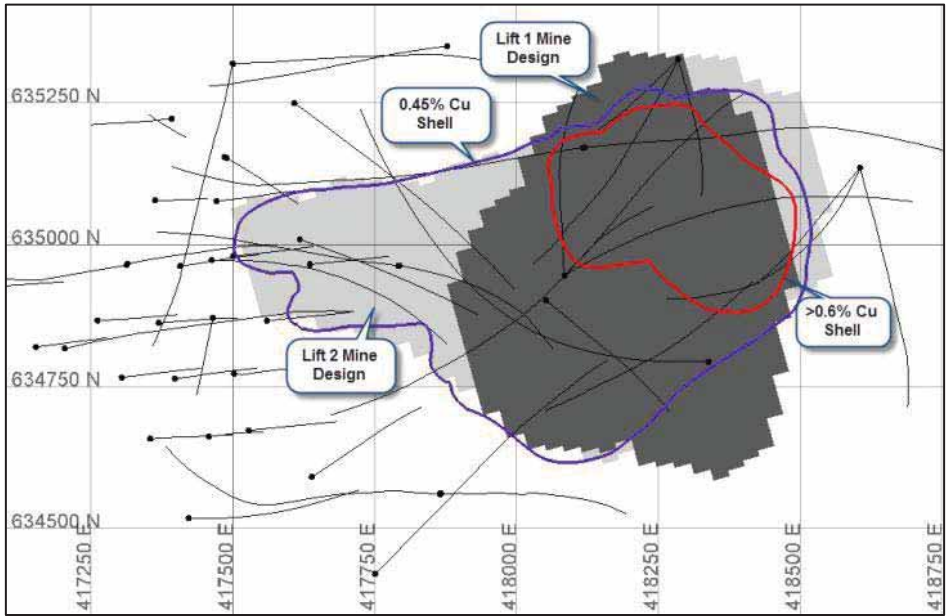
Figure 5. Nuevo Chaquiro Hypothetical Lifts in Grey Behind Grade Shells (Plan View)
