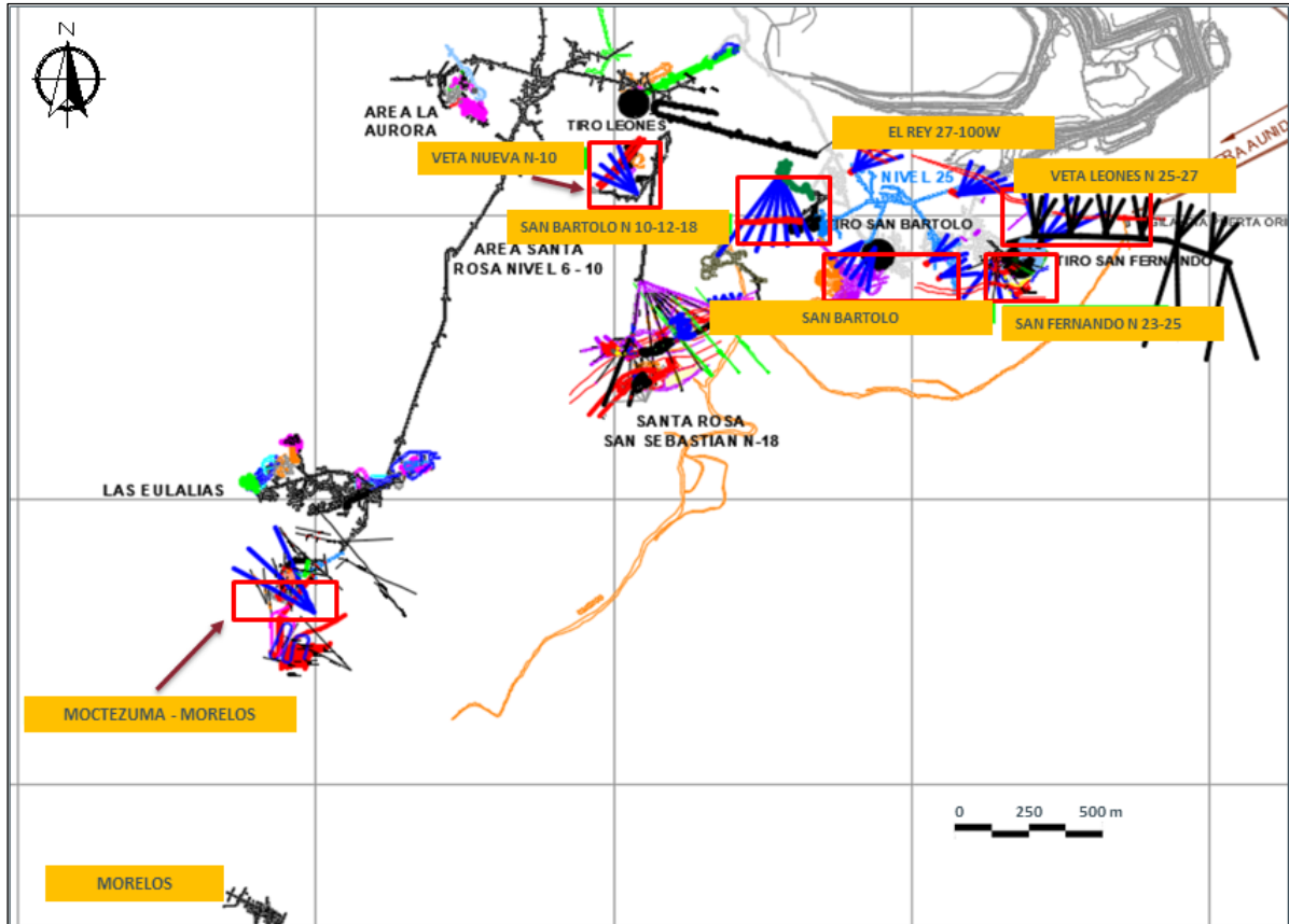
Figure 7-20: Location of Zones to Explore with Drilling from Underground and Surface
