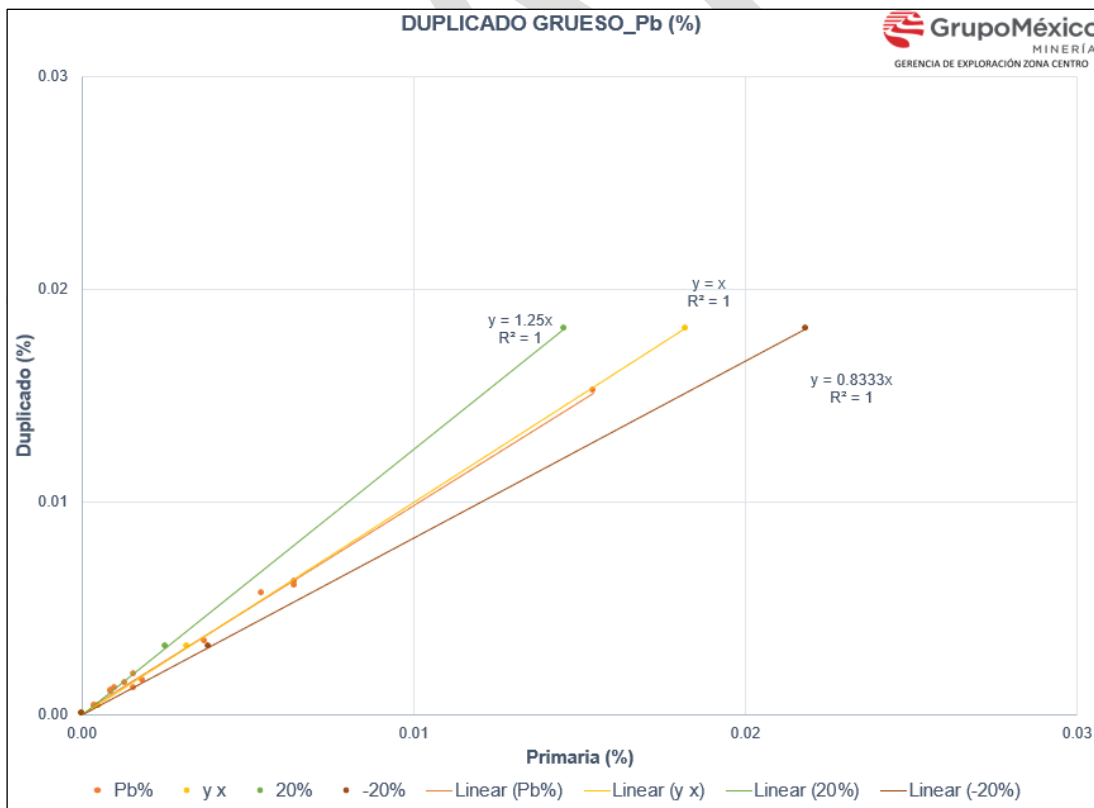
Figure 8-5: Graphs showing the Results in Scatterplots for Coarse Duplicate Controls (Ag and Pb)
