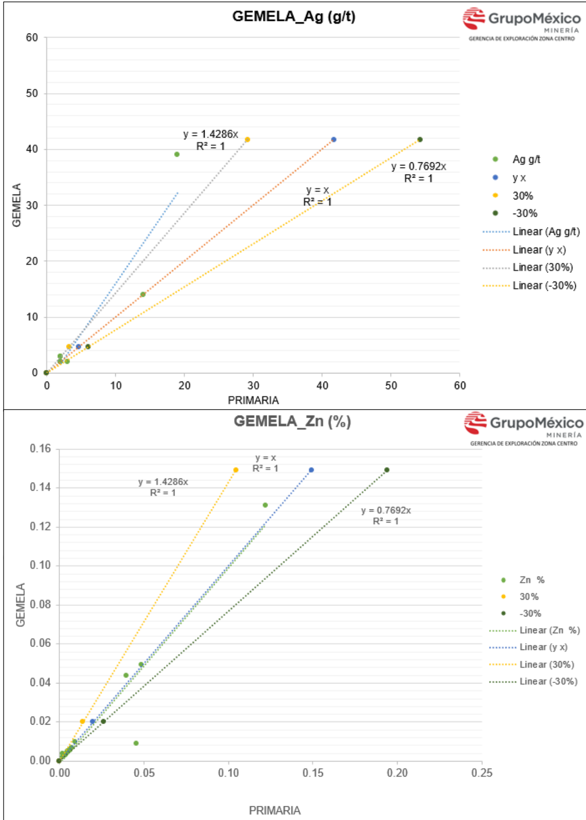
Figure 8-4: Graphs showing the Results of the Core Duplicate Controls (Ag and Zn)
