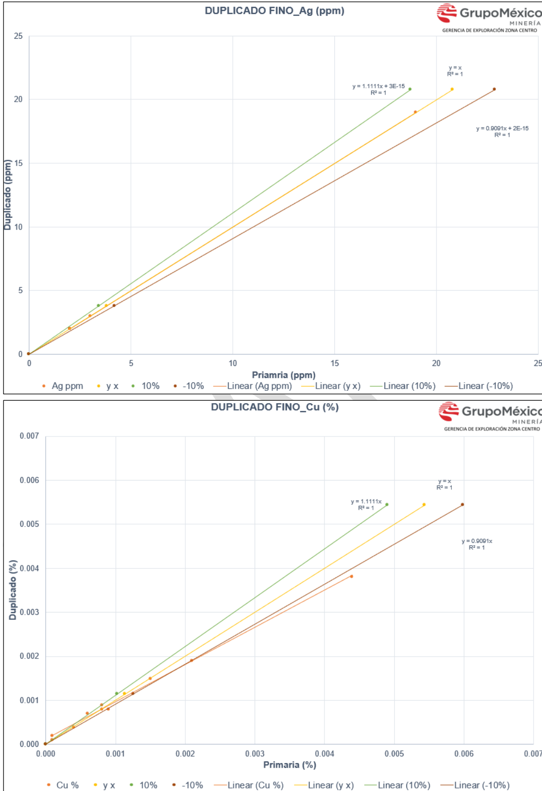
Figure 8-6: Graphs showing the Results in Scatterplots for Fine Duplicate Controls (Ag and Cu)
