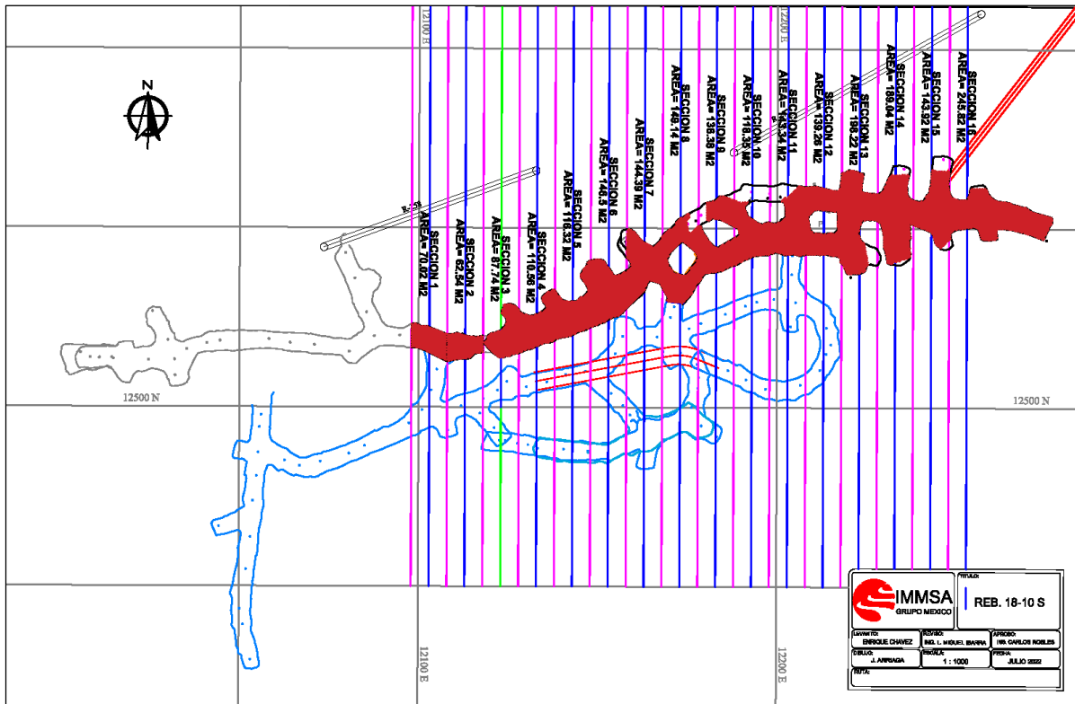
Figure 11-2: Example of Plan View Including the Calculated Areas of Mineralized Zones (Red Color), Reb 18-10S
