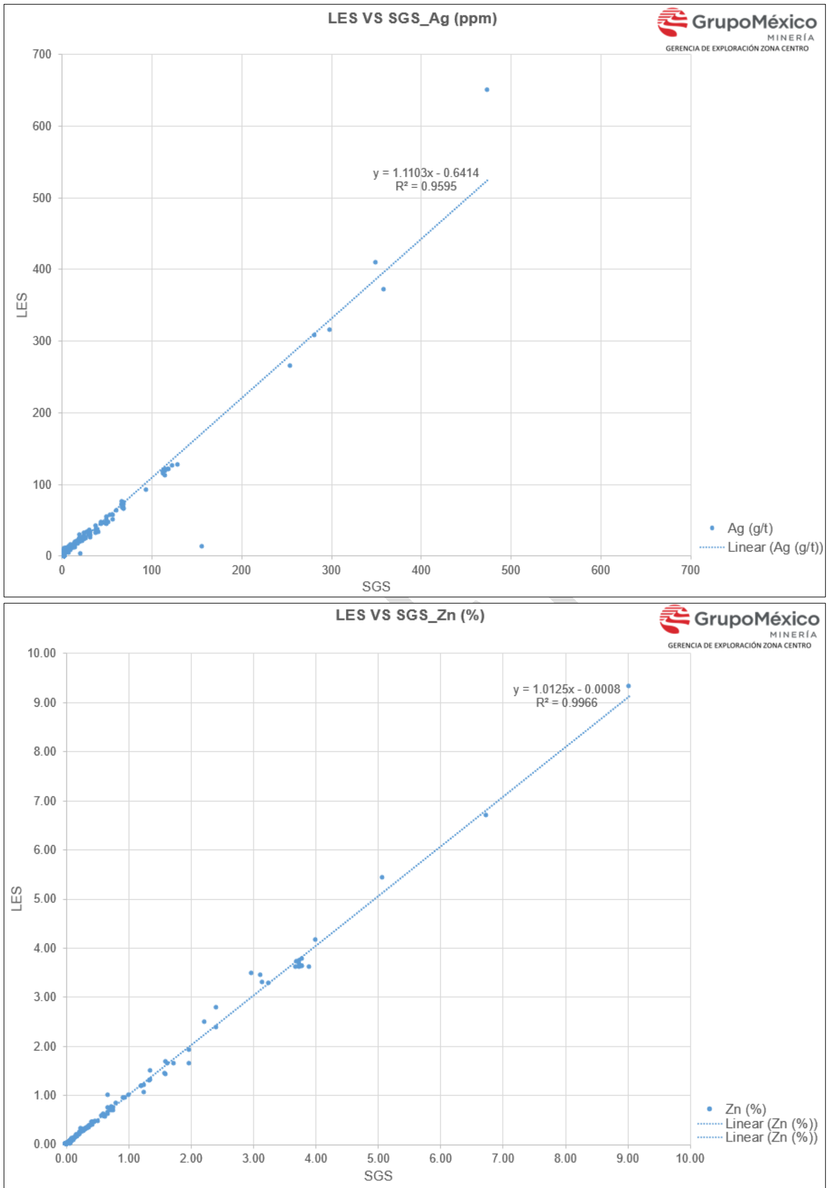
Figure 8-10: Scatterplots showing the Results of the Check Assays, SGS versus IMMSA Internal Laboratory (Ag and Zn)
