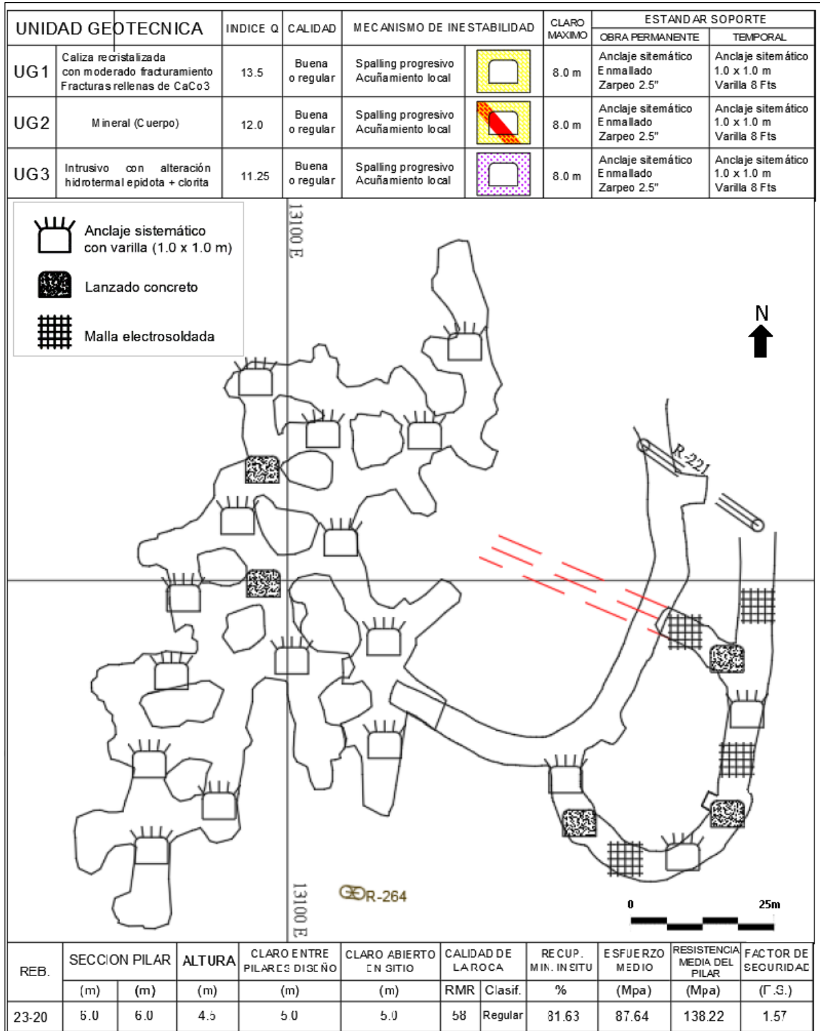
Figure 7-19: Example of the Geotechnical Evaluation of an Underground Location at Charcas
