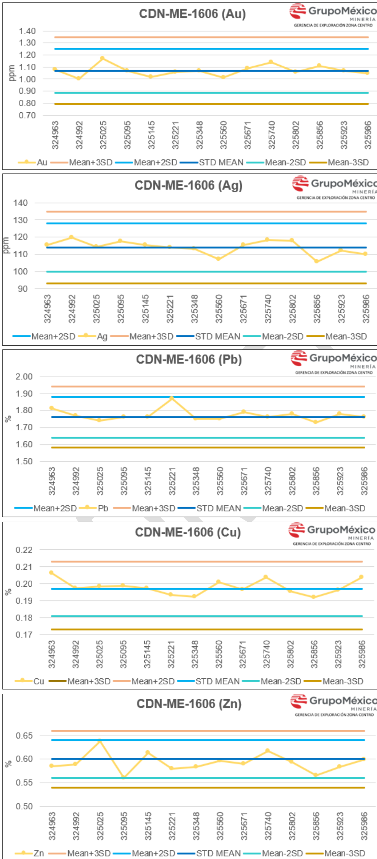
Figure 8-9: Graphs showing the Results of CDN-ME-1606 (Ag, Pb, Cu, and Zn)
