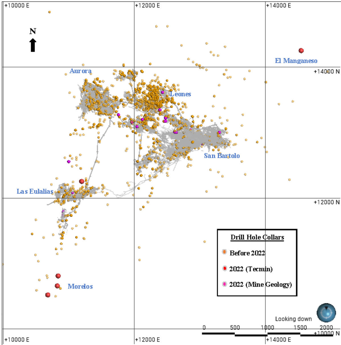
Figure 7-11: Location of Drillhole Collars at Charcas
