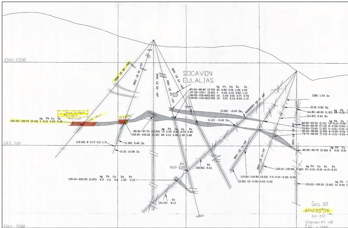
Figure 7-15: Example of a Mineralization Interpretation in a Vertical Section, Including the Core Sample Results
