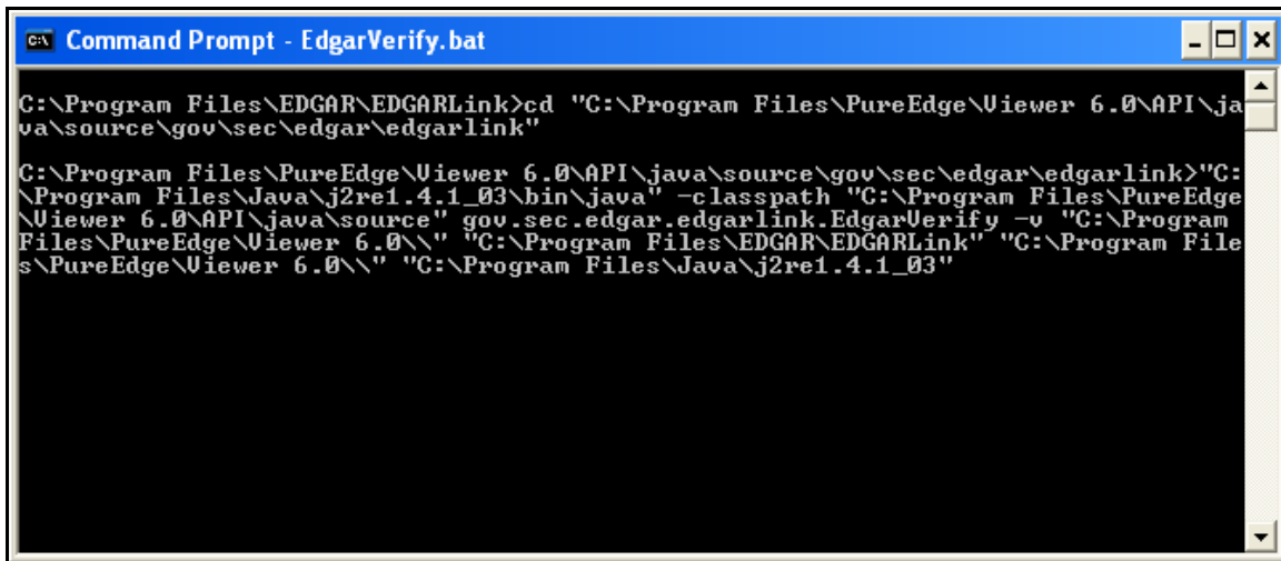
Figure 6-10: EDGARLink Integrity Check Window
